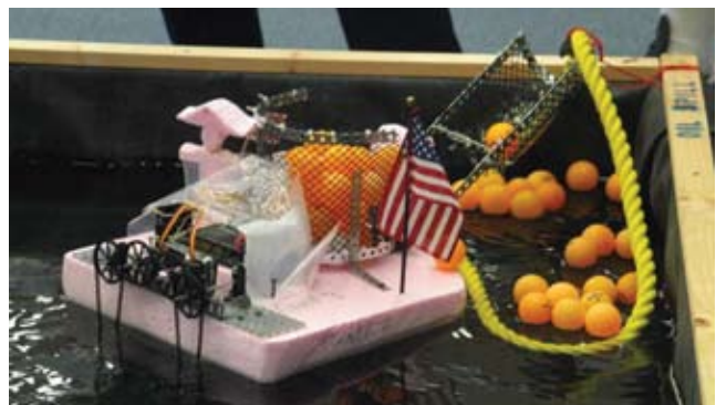
Robotic craft picking up the Ping-Pong ball “oil spill.”
